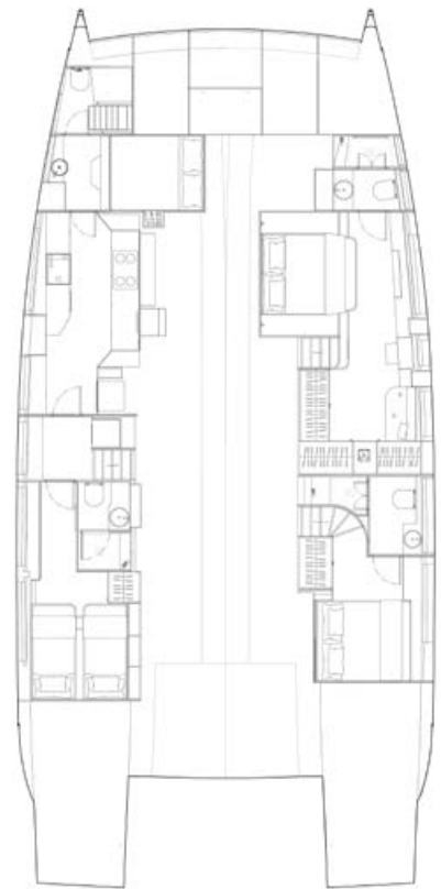
LOWER DECK 3 CABINS
