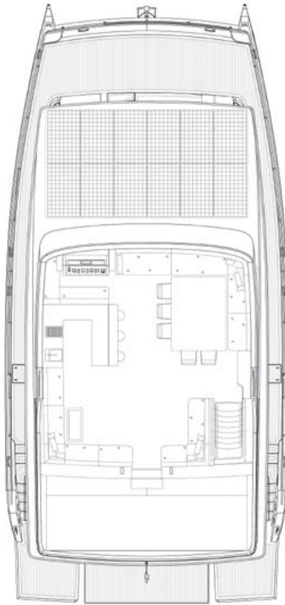
UPPER DECK 3-DECK OPEN
