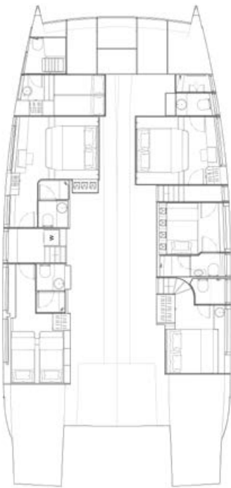
LOWER DECK 5 CABINS
