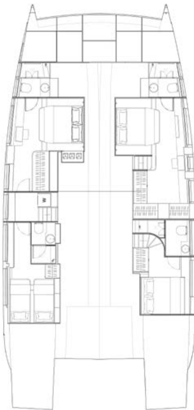
LOWER DECK 4 CABINS
