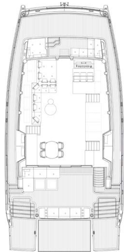
MAIN DECK 3-DECK FRONT EXIT - Alternative saloon layout
